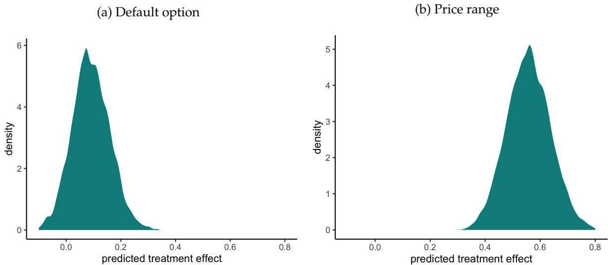
Figure D.4: Heterogeneous Treatment Effect Estimates and Standard Errors: Survival Forests
